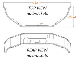
GY-0200-16 Step hole
